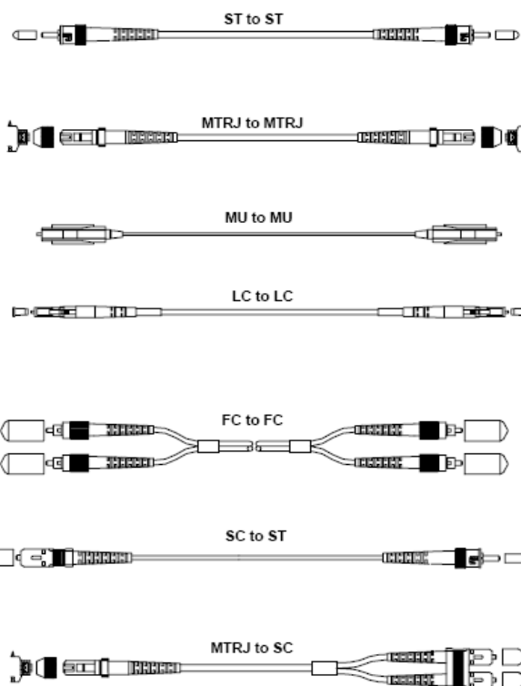
Fiber Optic Patch Cord
